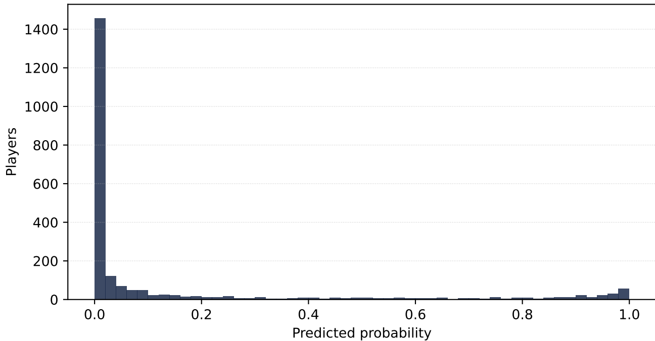
Stage 1 - Draft Classifier - Score Distribution
